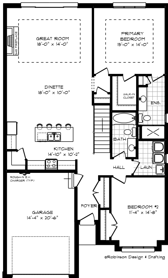
MAIN FLOOR PLAN 1529 SQ. FT.
