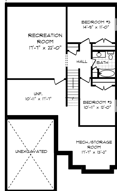
BASEMENT PLAN 865 SQ. FT. (finished)
